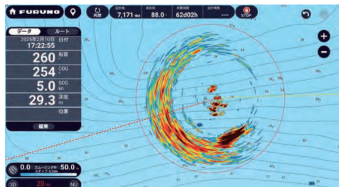
Overlaid sonar echo on chart display
