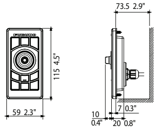
Remote Control Unit MCU-002 (option) 0.14 kg 0.3 lb
