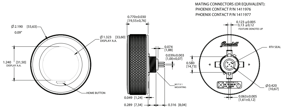
Touch Encoder Unit TEU001B/S
