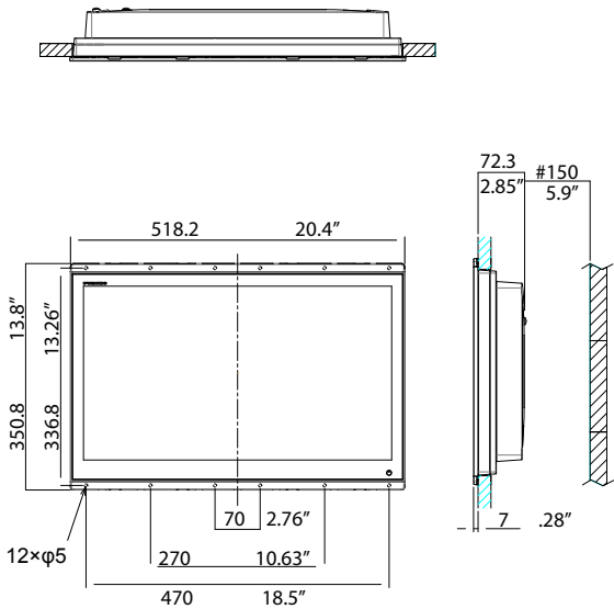
TZT22X (Flush Mount) Cutout Dimension
