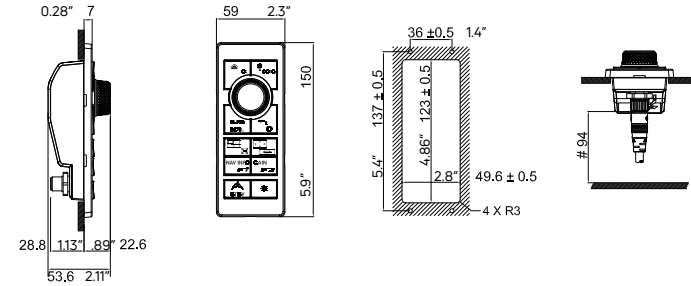
Control Unit MCU-006 (option)
