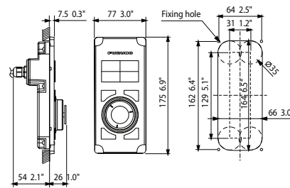
Remote Control Unit MCU-004 (option) 0.4 kg 0.9 lb
