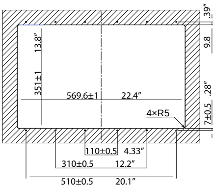
TZT24X (Flush Mount) Cutout Dimension
