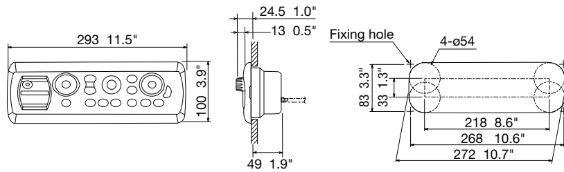
Control Unit MCU-005 (option)
