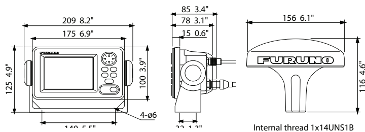
Display Unit NX-300
