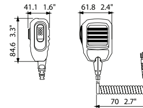
Microphone MIC-5000
