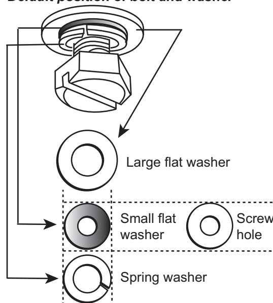
Default position of bolt and washer
