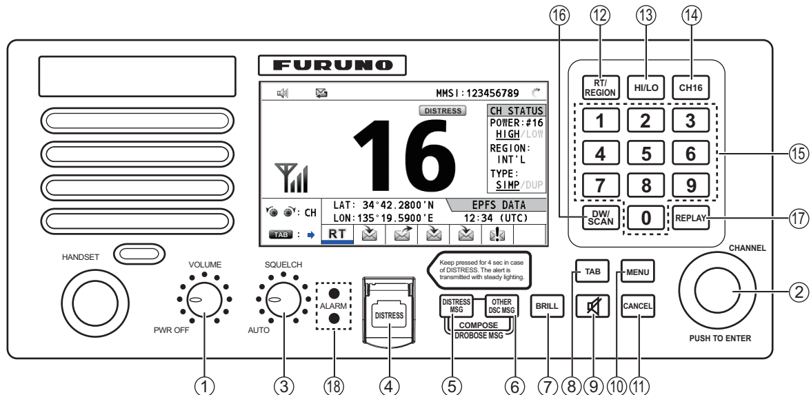
Transceiver unit
